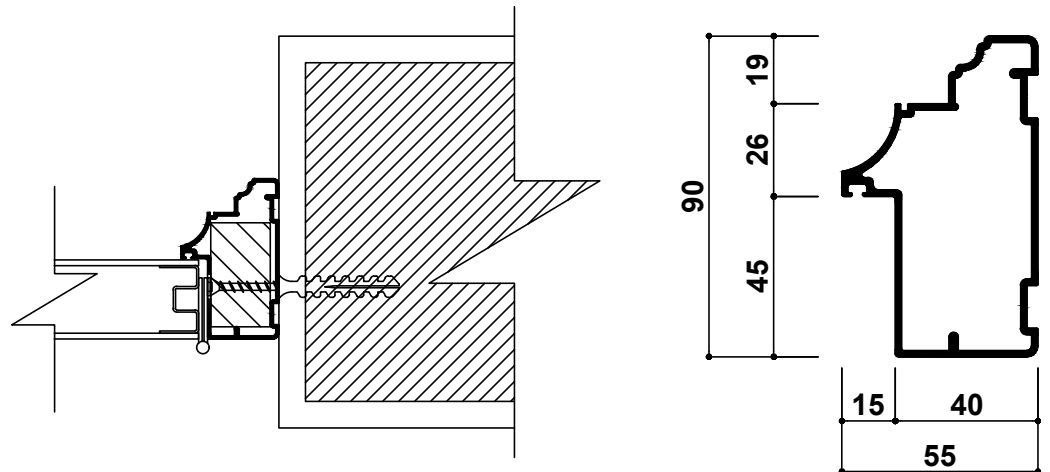
CT-01
