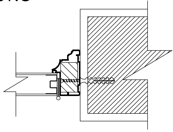
CT-01
