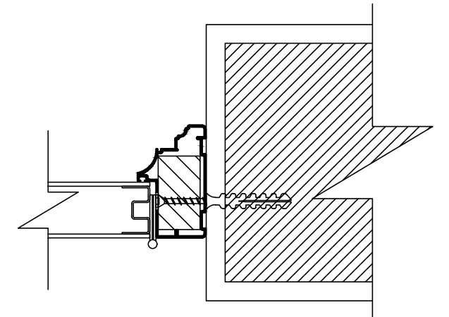
CT-01
