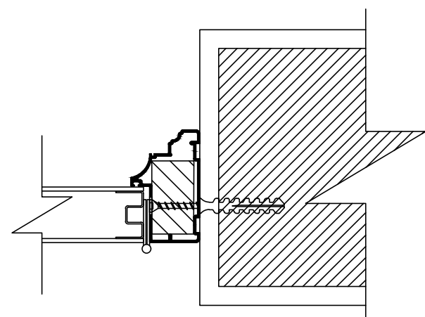
CT- 01
